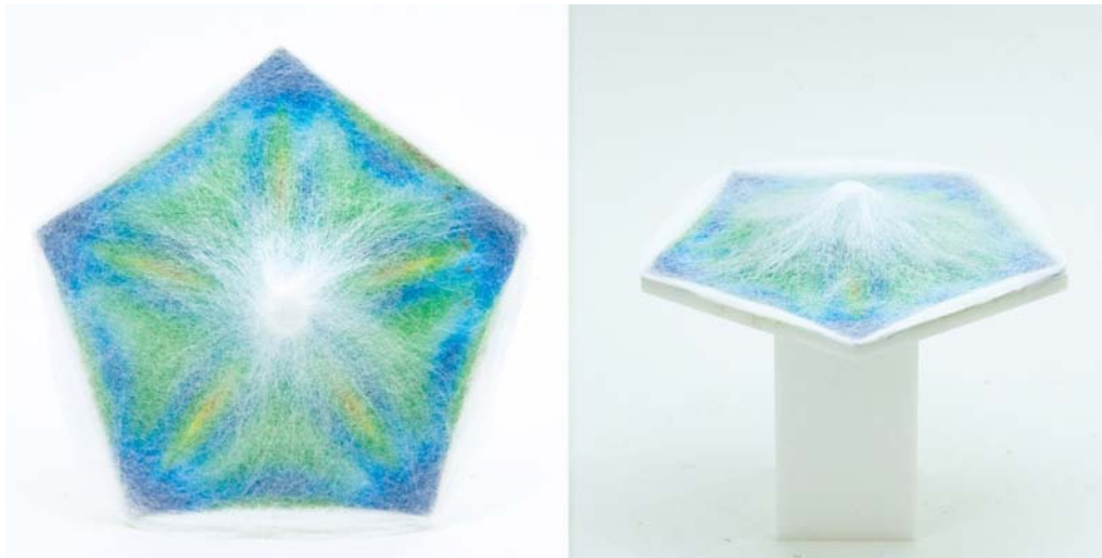
Figure 10 One-dice polygonal platforms showing greater density of silk deposition in areas of higher Stress-Strain.
