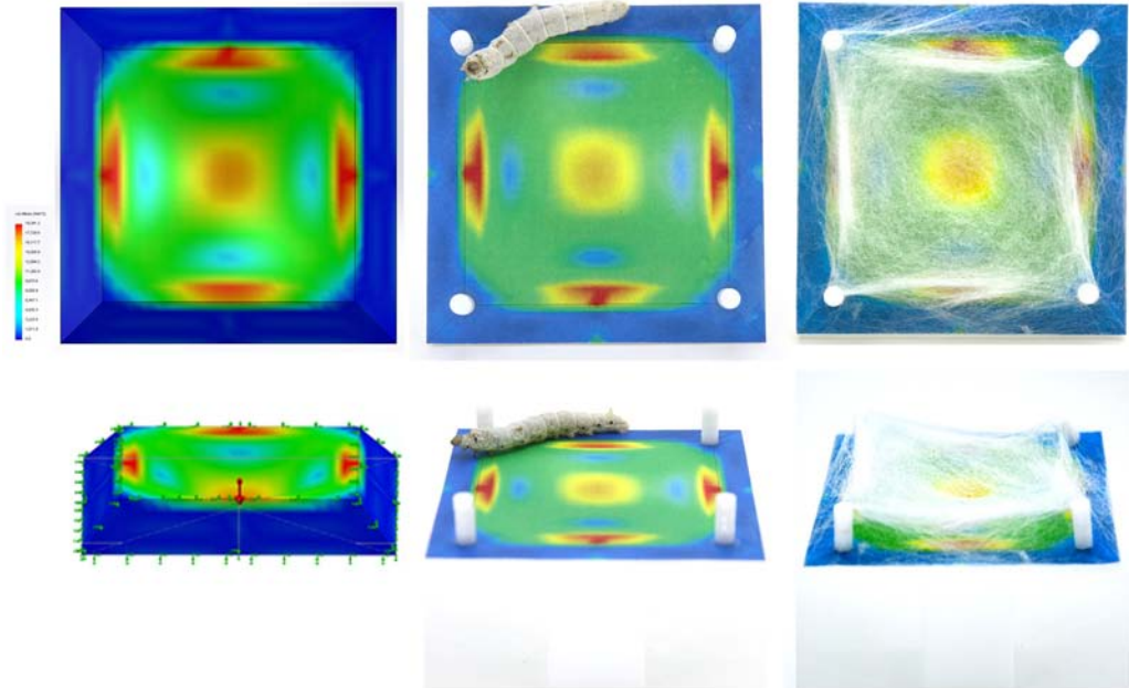
Figure 8 4-Dice face configurations. L to R: Digital representation of anticipated stress for membrane structure based on 4 poles calculated within SolidWorks; physical model with digital representation as base. The silkworm is shown to the right; physical model juxtaposed with silk fibre by the Bombyx mori silkworm. Denser fibres appear between poles along boundaries as anticipated by the FEM model.
